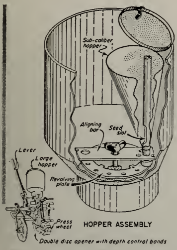
SMALL SEED ATTACHMENT FOR DRILL
